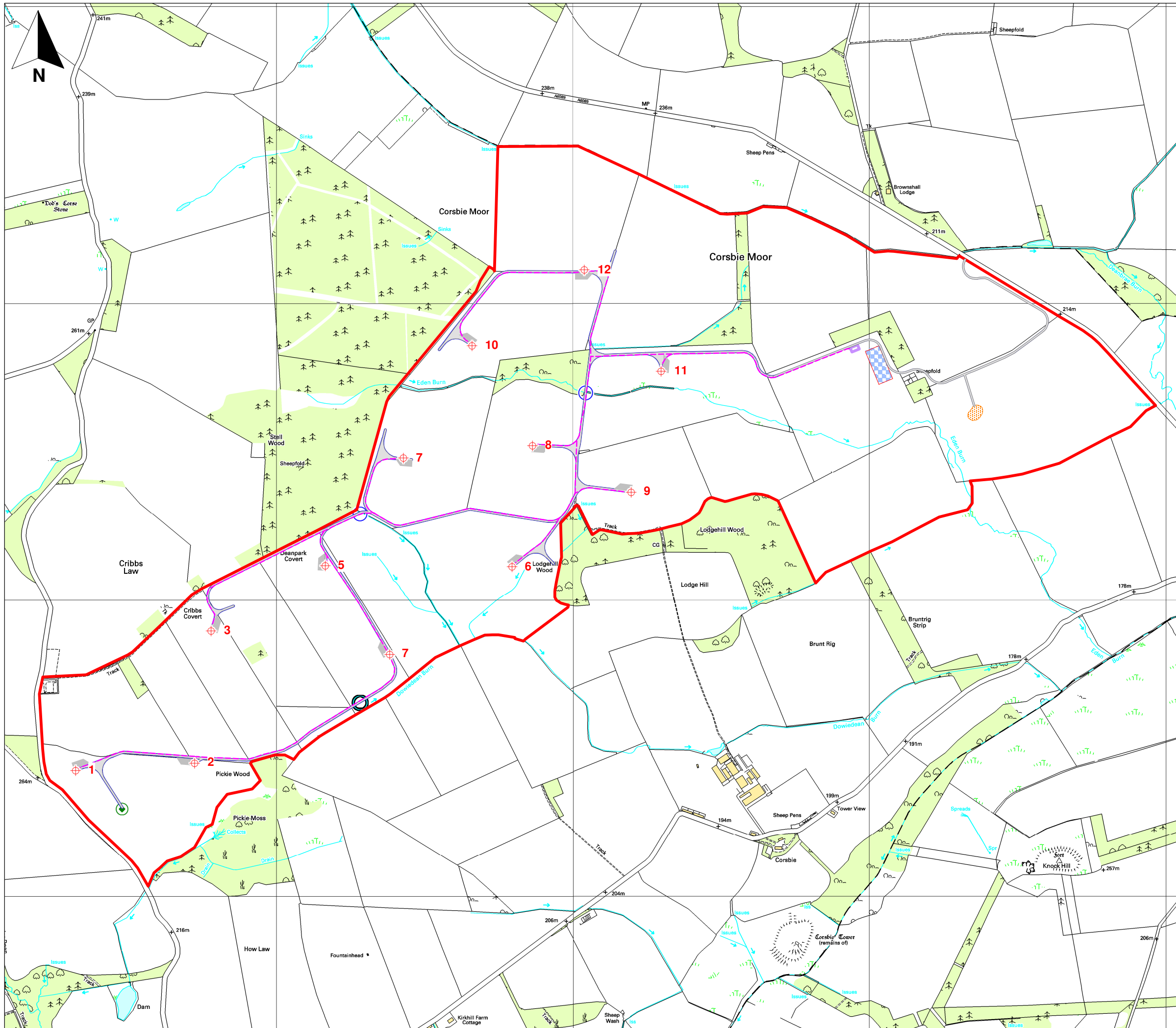
Figure 3.1 DRAFT Site Layout 16 February 2011
